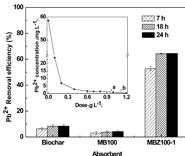
Figure 8. Removal efficiency of Pb (II) by three sorbents (biochar, MB100, and MBZ100-1) at 7, 18, and 24 h. Experiment conditions: initial concentration 100 mg L -1 (50 mL), sorbent 10 mg, pH 6, and temperature 25 °C. Inset is the treatment capacity of MBZ100-1 for the Pb (II) solution. Experiment conditions: initial concentration 60 mg L -1 , sample dose 0.1–1.2 g of sorbent/L of Pb (II) solution volume, pH 6, temperature 25 °C, and contact time 22 h. Panels a and b represent the waste discharge standard regulated by GB 8978-1996 and the EPA, respectively.
