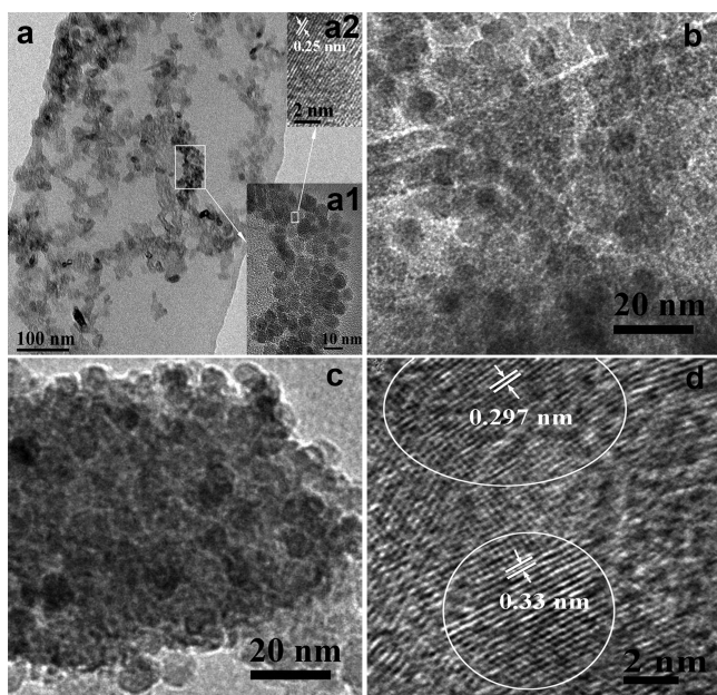
Figure 3. TEM images of composites: (a) TEM images of MB100 (insets a1 and a2 are the enlarge image and HRTEM image of the selected area, respectively), (b) TEM image of MBZ100-0.5, (c) TEM image of MBZ100-1, and (d) HRTEM image of MBZ100-0.5.
