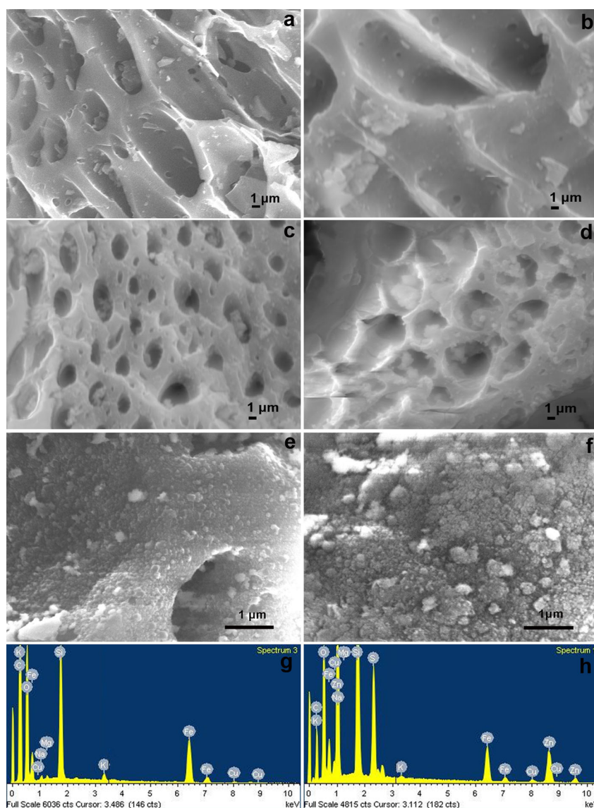
Figure 2. SEM images and EDX results of composites: (a) SEM image of biochar ( \times 3000 ), (b) SEM image of MB100 ( \times 3000 ), (c) SEM image of MBZ100-0.5 ( \times 3000 ), (d) SEM image of MBZ100-1 ( \times 3000 ), (e) SEM image of MBZ100-0.5 ( \times 20,000 ), and (f) SEM image of MBZ100-1 ( \times 20,000 ). EDX results of selected areas of (g) MB100 and (h) MBZ100-1.
