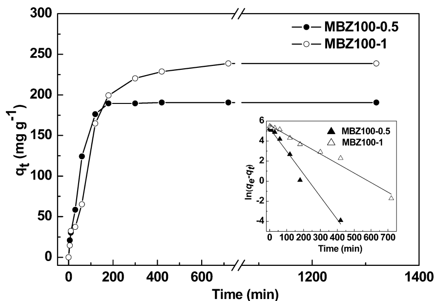
Figure 5. Adsorption kinetics of Pb (II) on magnetic biochar/ZnS composites. Inset is fitting of the pseudo-first-order model. Symbols are experimental data. Solid lines represent the fitted curves. Experiment conditions: initial concentration 100 \text{ mg L}^{-1} (50 mL), sorbent 20 mg, pH 6, temperature 25 \text{ }^{\circ}\text{C} , and contact time 22 h.
