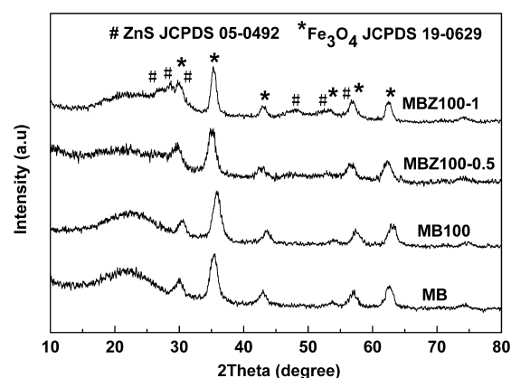
Figure 1. XRD patterns of MB, MB100, MBZ100-0.5, and MBZ100-1.
