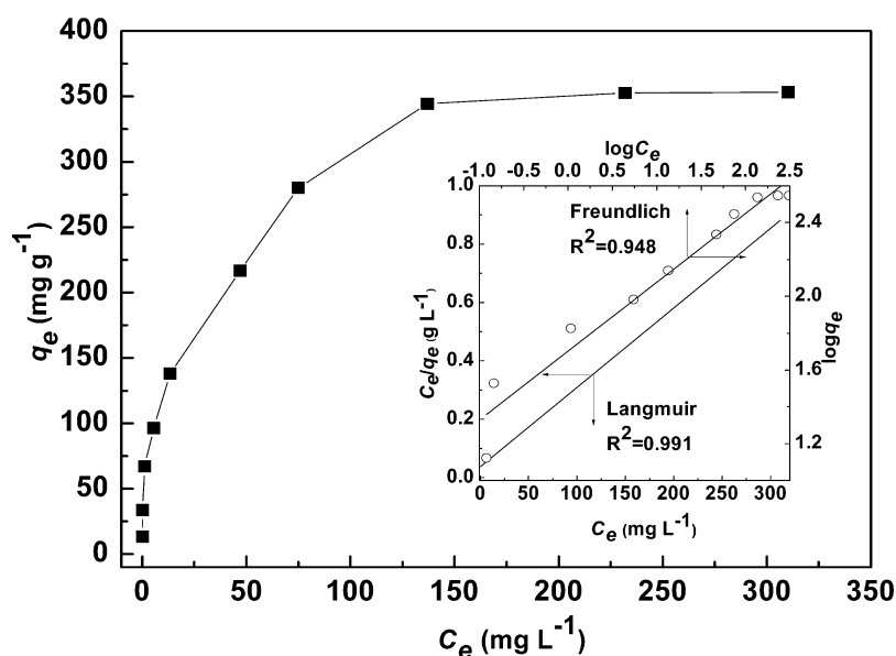
Figure 6. Adsorption isotherm of Pb (II) on MBZ100-1. Inset is fitting of Langmuir and Freundlich models. Symbols are experimental data. Solid lines represent the fitted curves. Experiment conditions: initial concentration 20–700 \text{mg L}^{-1} (50 mL), sorbent 60 mg, pH 6, temperature 25 \text{ }^{\circ}\text{C} , and contact time 24 h.
