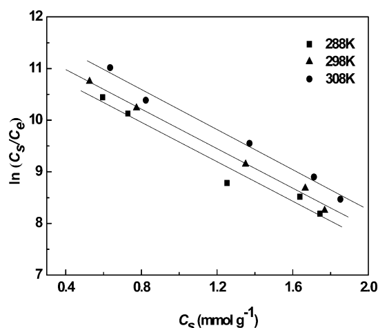
Figure 9. Plots of \ln(C_s/C_e) vs C_s at 288, 298, and 308 K. Experiment conditions: initial concentration 75–300 mg L -1 (50 mL), sorbent 30 mg, pH 6, and contact time 24 h.
