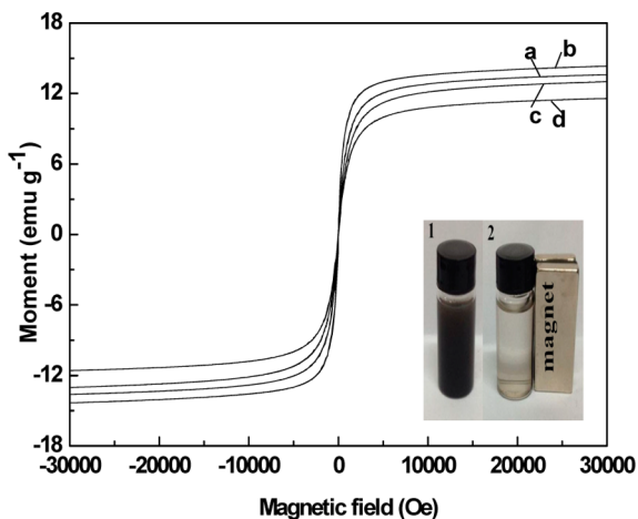
Figure 4. Magnetization curves of composites at 300 K: (a) MB, (b) MB100, (c) MBZ100-0.5, and (d) MBZ100-1. Inset is the photograph of dispersion of MBZ100-0.5 in aqueous solution (1) and its response to a magnet (2).
